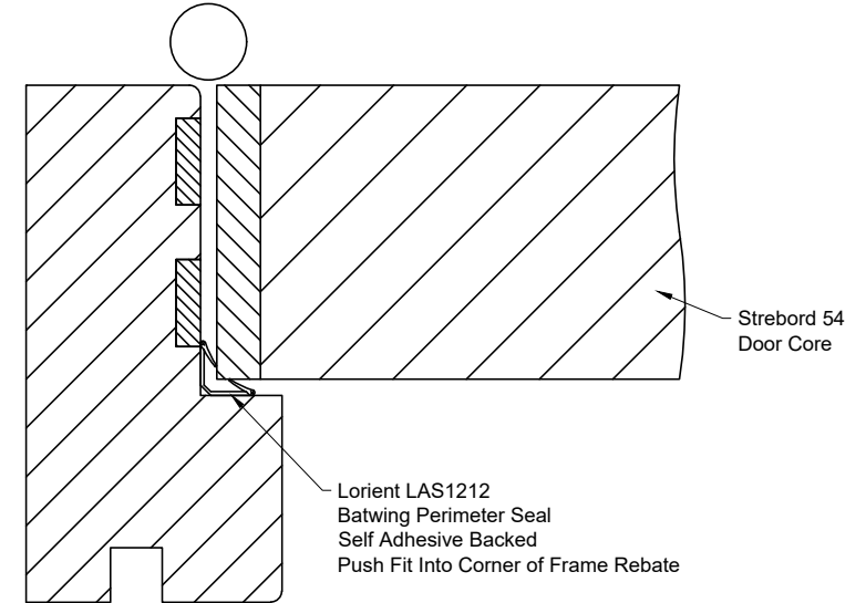
Streborb 54 FD60 PAS24 Doorset With Lorient LAS1212 Batwing Perimeter Seal
