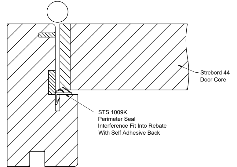
Streborb 44 FD30 PAS24 Doorset With STS 1009K Perimeter Seal
