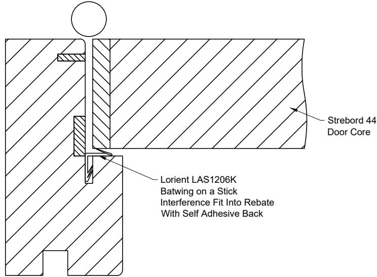
Streborb 44 FD30 PAS24 Doorset With Lorient LAS1206K Batwing on a Stick
