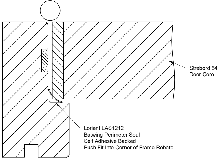
Streborb 54 FD30 PAS24 Doorset With Lorient LAS1212 Batwing Perimeter Seal
